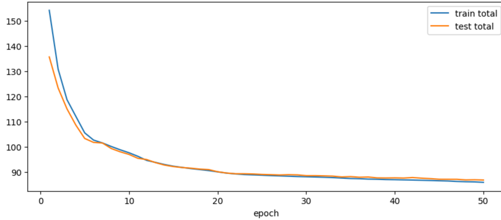
FC-VAE Reconstruction Loss
