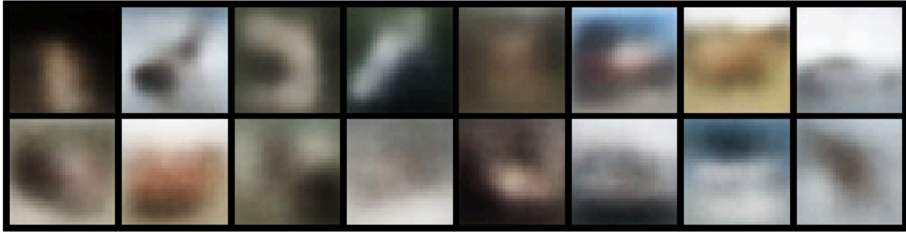
Generated samples: Conv-VAE (top) vs FC-VAE (bottom)
